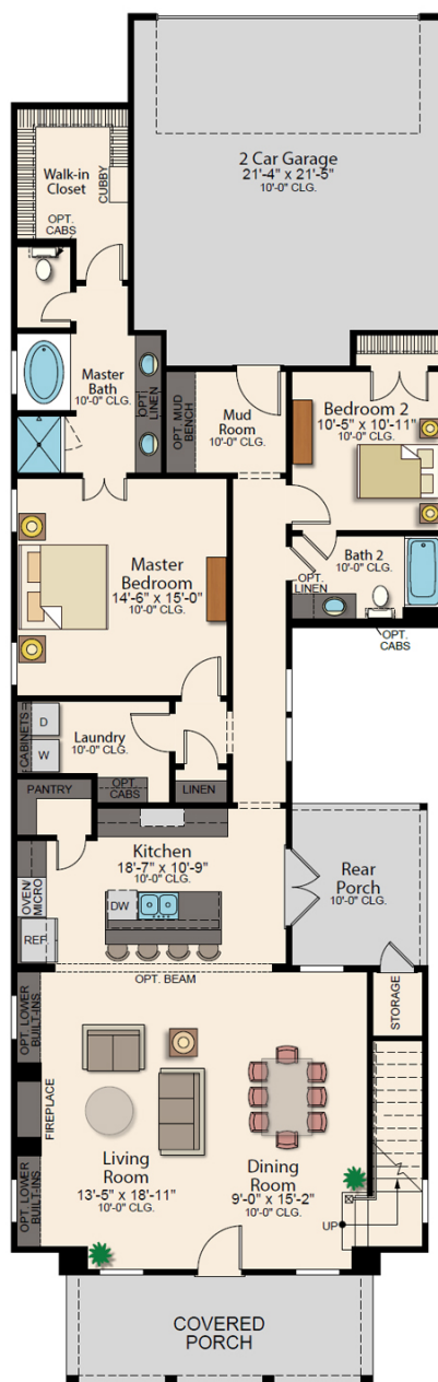
FIRST FLOOR
