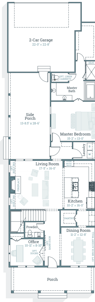
FIRST FLOOR
